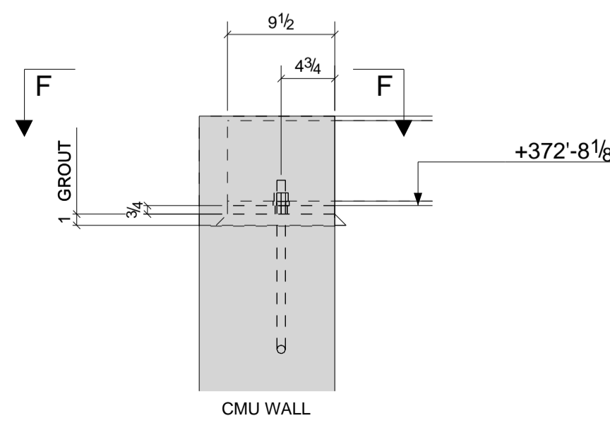
DETAIL C
